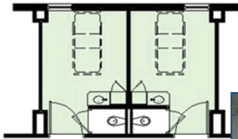
Existing Layout
